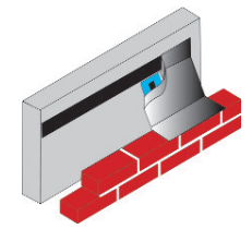
Cavity Tray Bonded to Joint Support
